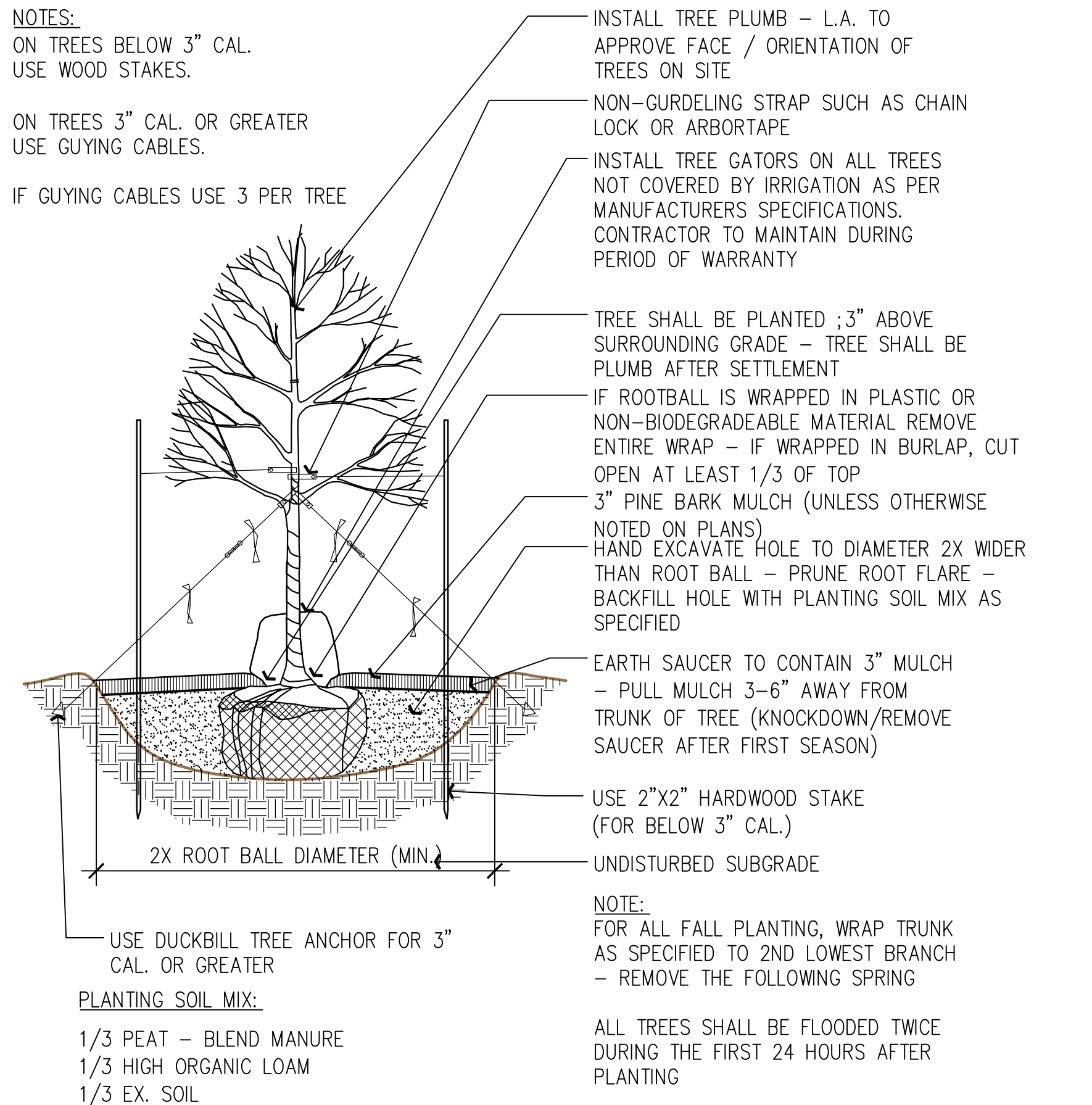
SHADE / FLOWERING TREE DETAIL NTS
