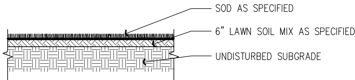
SOD LAWN DETAIL NTS
