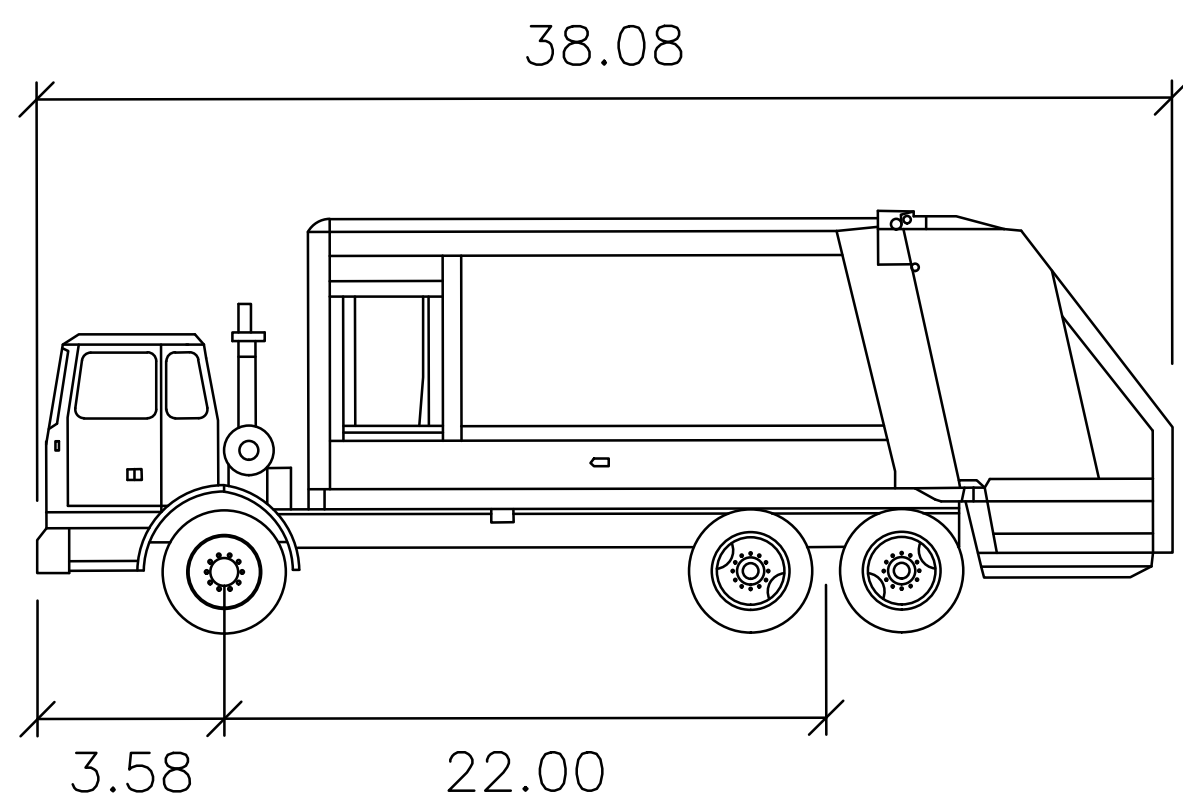
REAR-LOAD GARBAGE TRUCK
