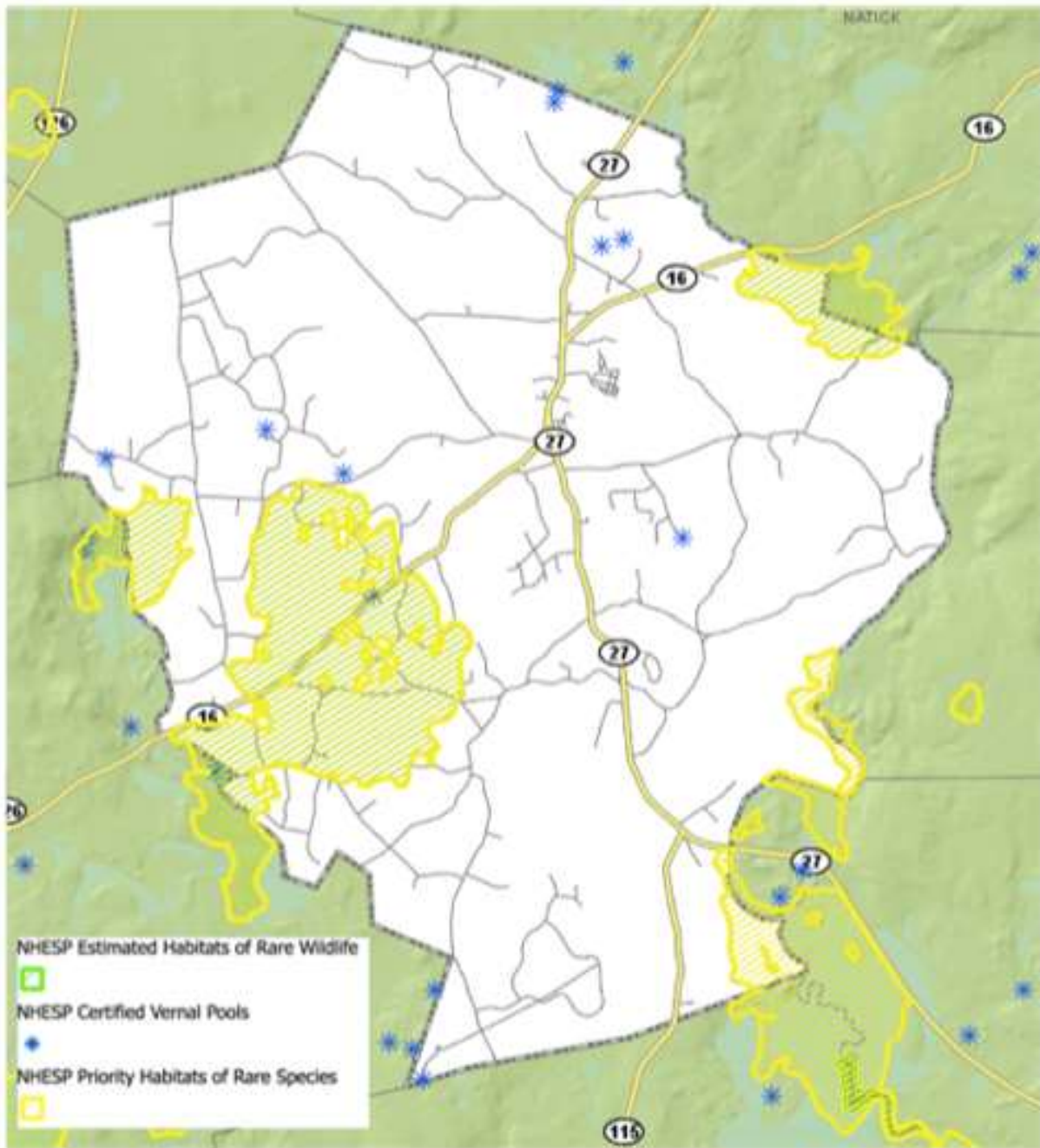
MAP 4.8 — Priority and estimated habitat of rare and endangered species and state-certified vernal pools
