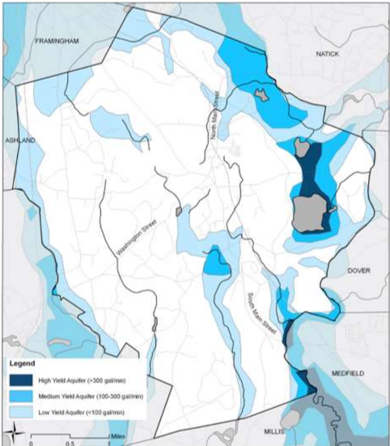
MAP 4.5—Aquifers: Sherborn's only high-yield aquifers lie in the Farm Pond area and along the Charles River, both on the eastern side of town. In general, the town has limited underground water resources.
