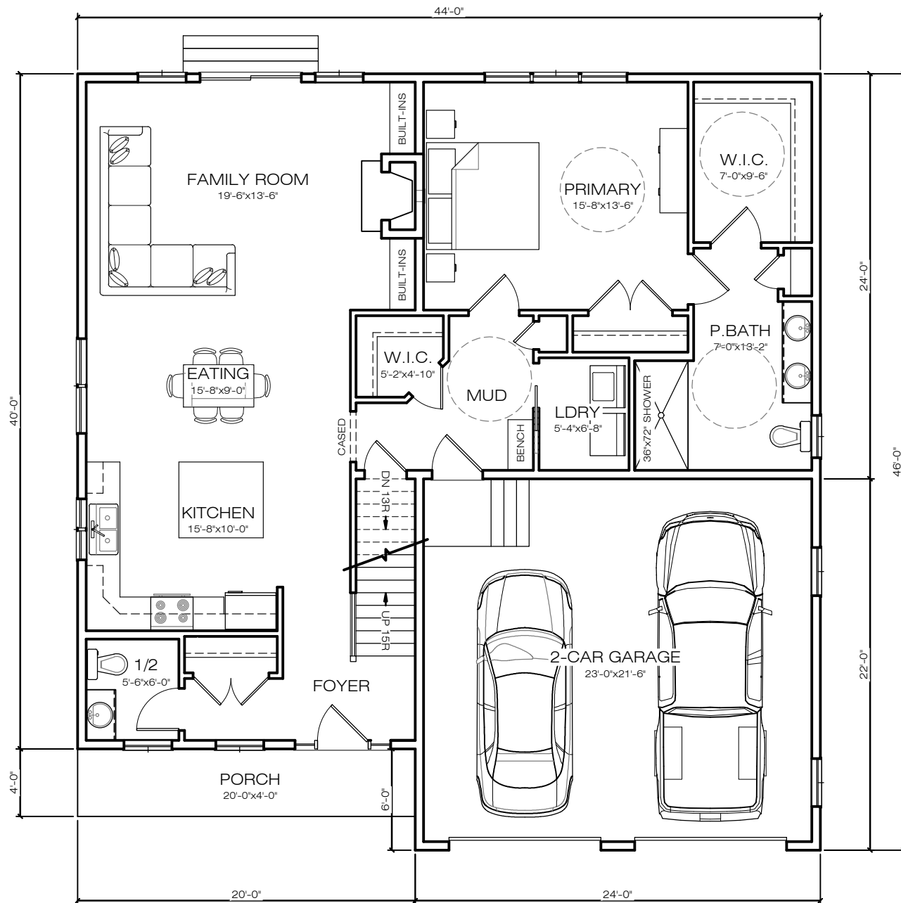
FIRST FLOOR PLAN 9'-0" CEILING HEIGHT 1,384 SQ. FT.
